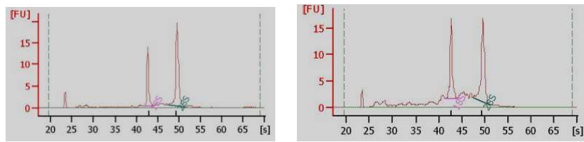
Fig. 2 Total RNA was analyzed by Agilent bio-chip
