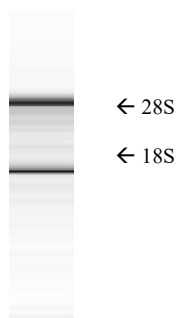
Fig. 1 Total RNA was analyzed by Agilent bio-chip
